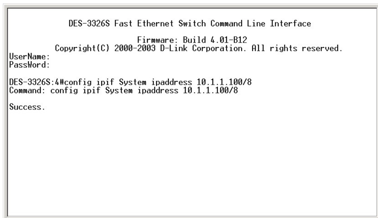
Figure 2 - 3. Assigning the Switch an IP Address
